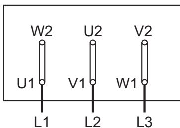
△ – Connection 230 V (400 V)
