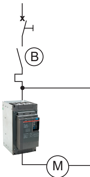
Alternative B Main contactor located outside the delta circuit
