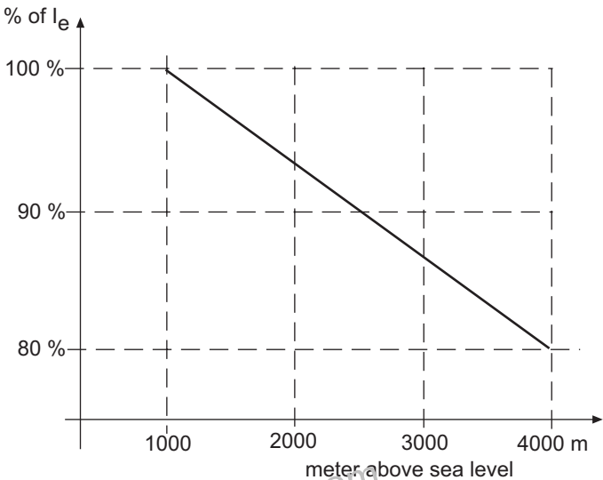
Derating of motor current at high altitudes
