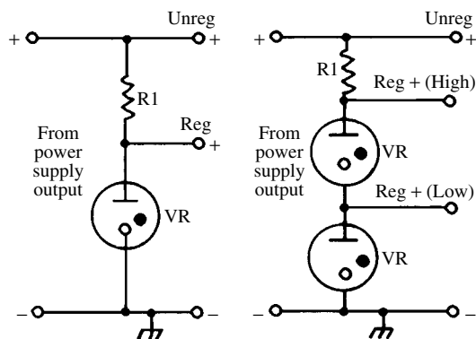
L-type voltage regulator
