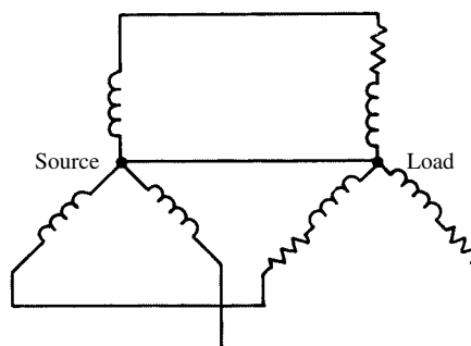
wye-wye circuit
