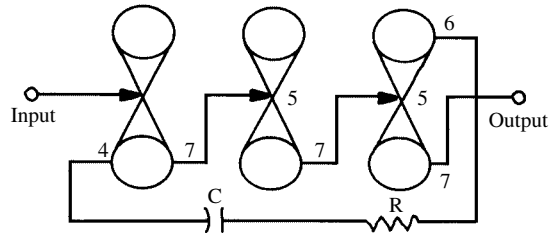
divide-by-seven circuit
