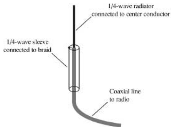
coaxial antenna
