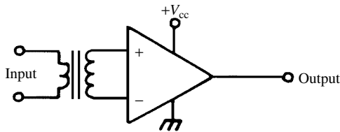
open loop, 2.
