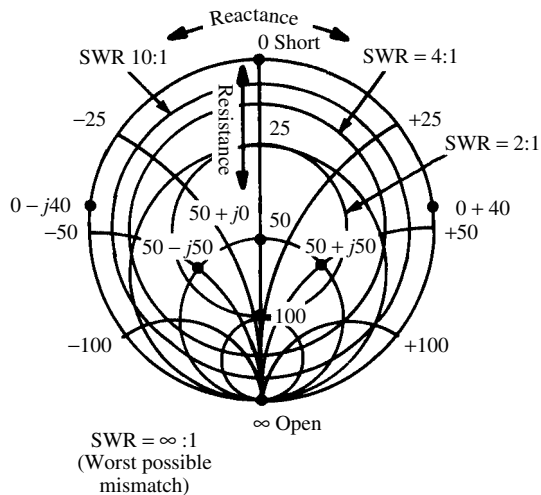
Smith chart
