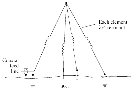
Alexanderson antenna
