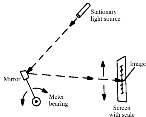
optical lever
