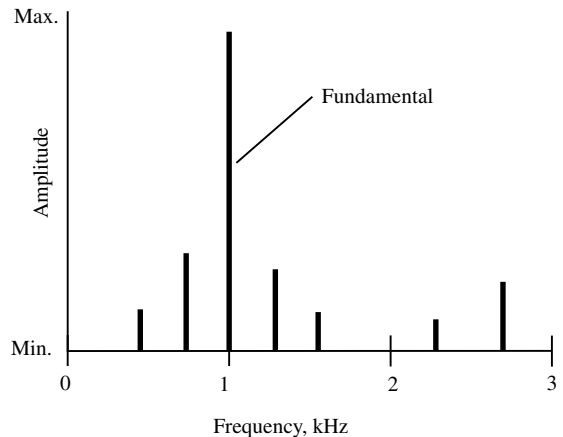
inharmonic distortion
