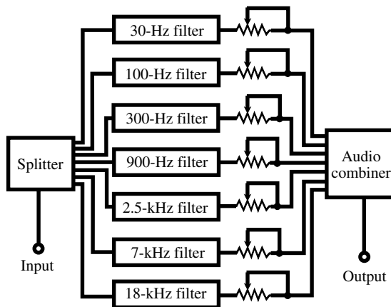
graphic equalizer
