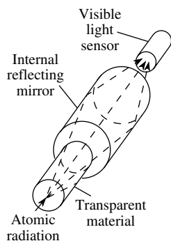
Cerenkov radiation
