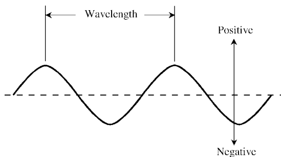
wavelength
