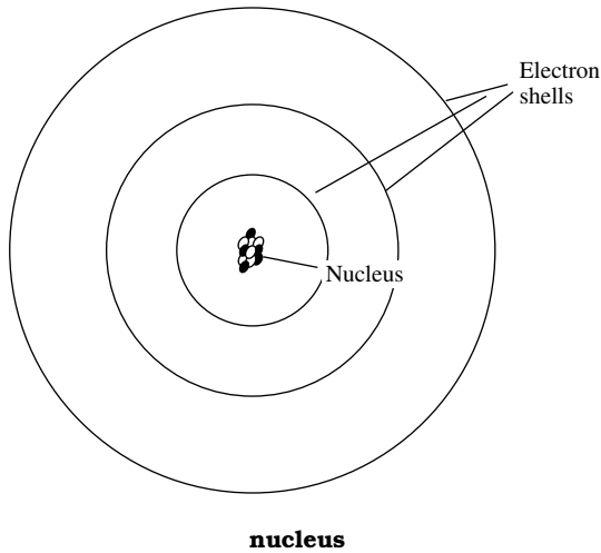
nucleus
