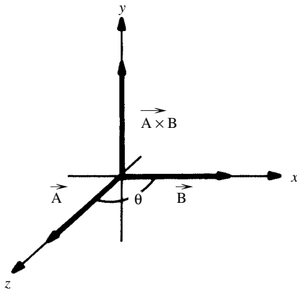
cross product
