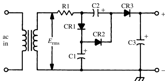
tripier, 1
