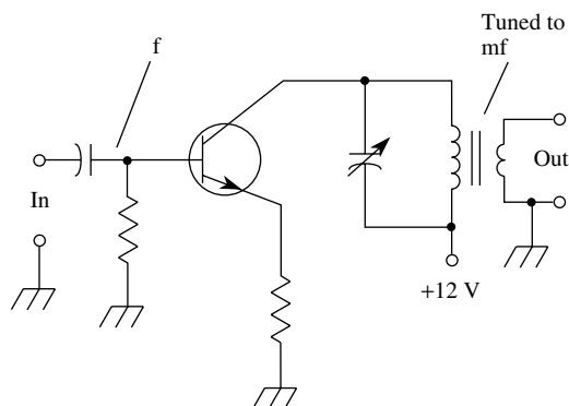
multiplier amplifier
