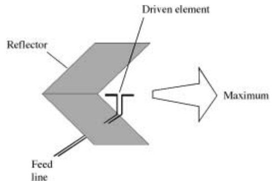
corner-reflection antenna
