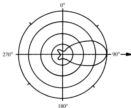
unidirectional pattern
