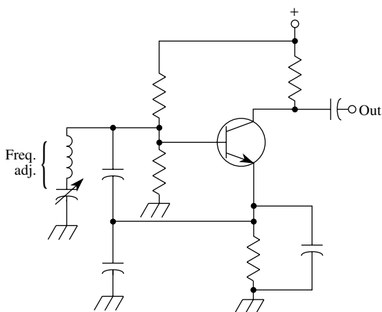
Clapp oscillator
