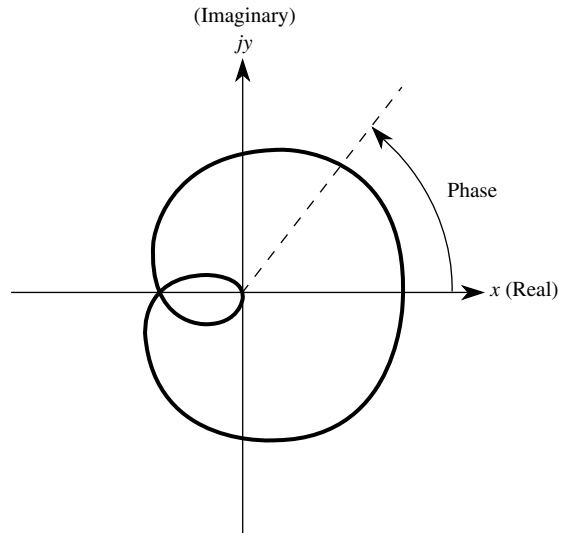
Nyquist diagram
