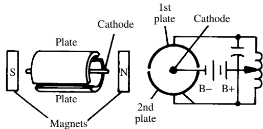
magnetron
