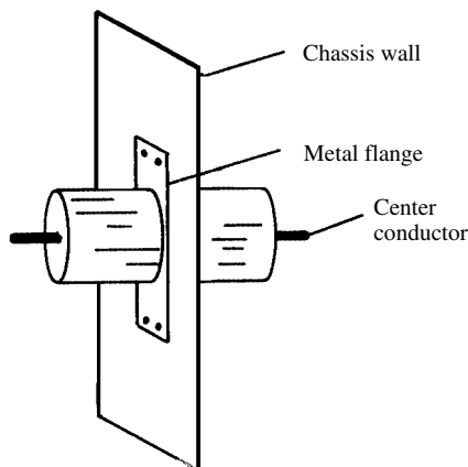
feedthrough capacitor
