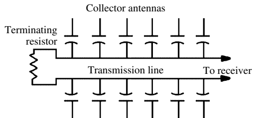
fishbone antenna
