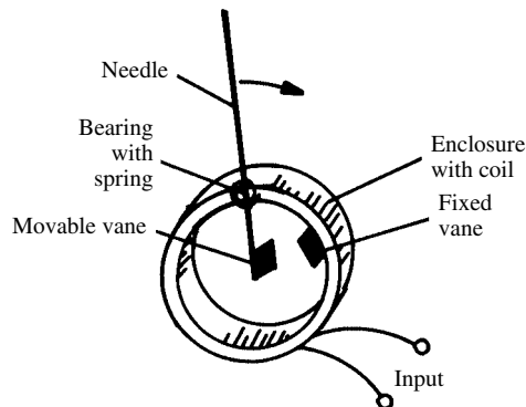
iron-vane meter
