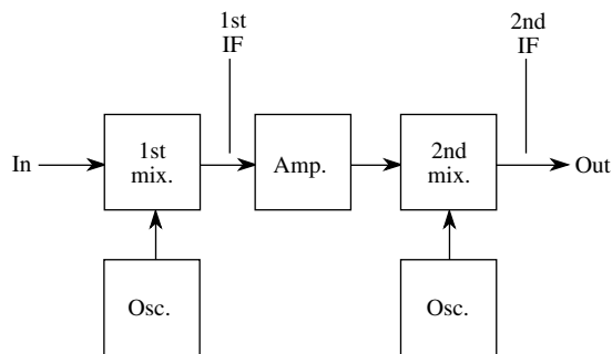
double conversion
