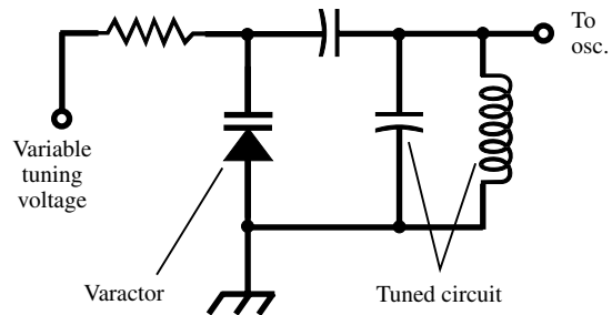
electric tuning
