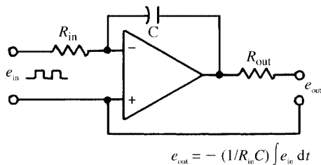
analog integrator
