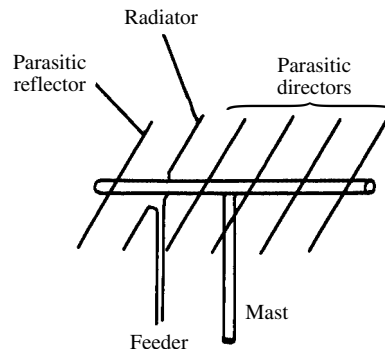
yagi antenna
