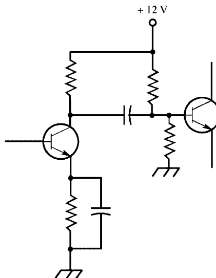
bypass capacitor
