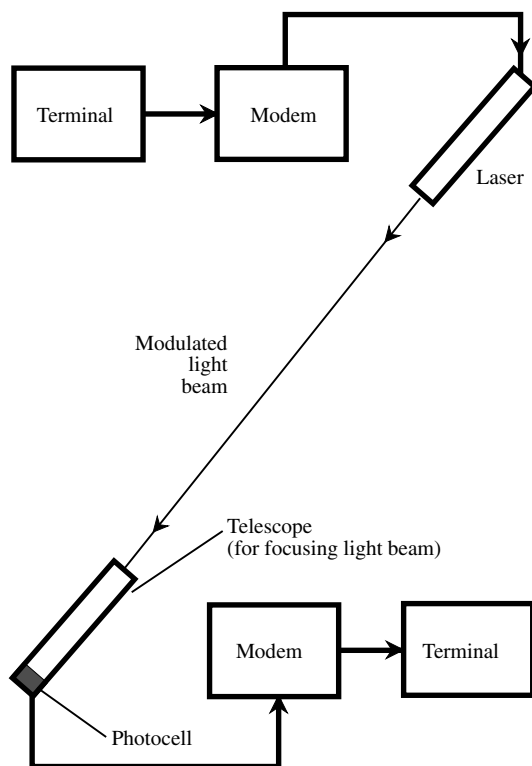
light-beam communication
