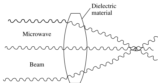
dielectric lens
