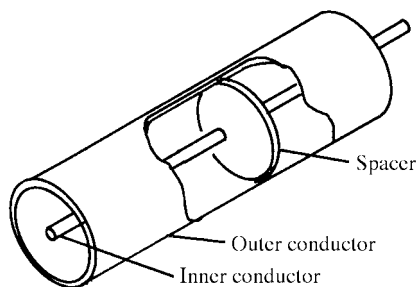
air-dielectric coax
