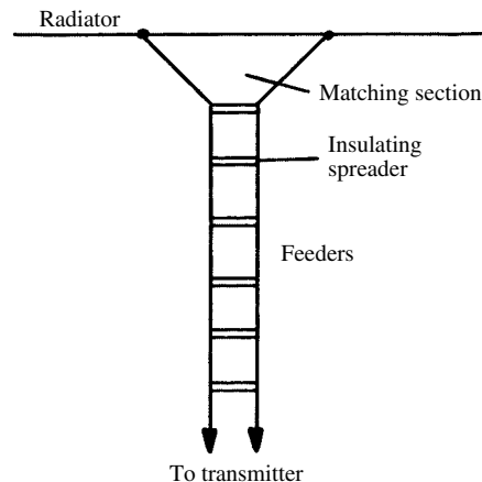
wye-matched-impedance antenna
