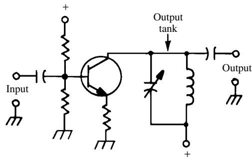
output tank
