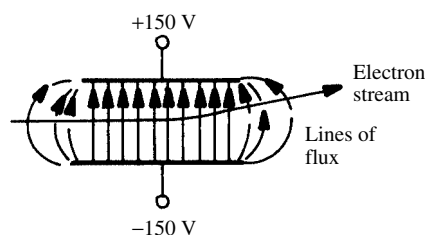
electrostatic deflection
