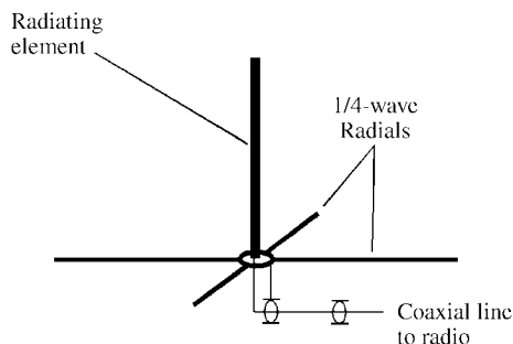
ground-plane antenna
