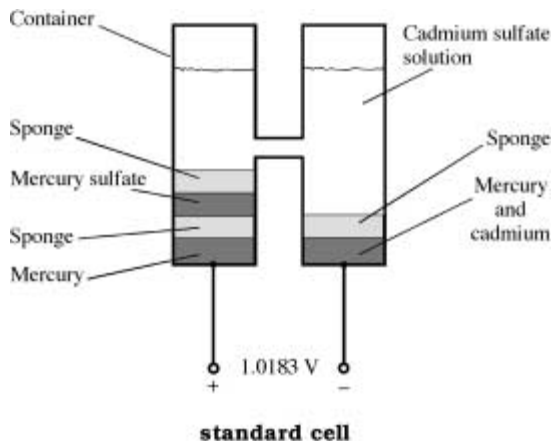
standard cell
