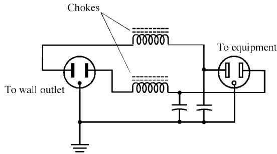
line filter
