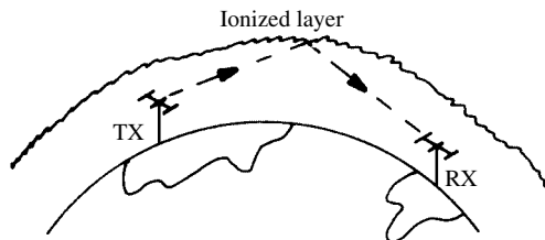
indirect wave
