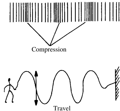
elastic waves
