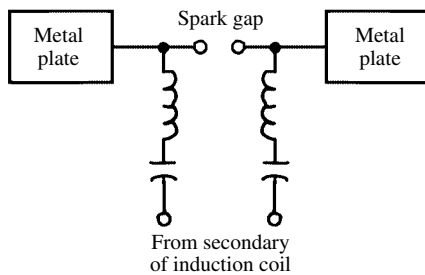
Hertz oscillator
