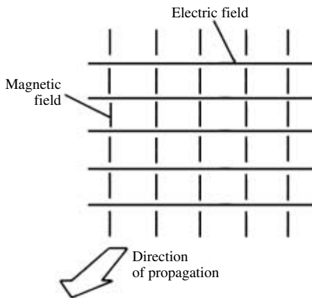
electromagnetic field
