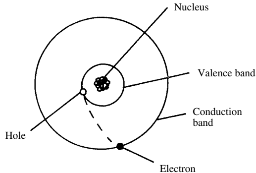
electron-hole pair
