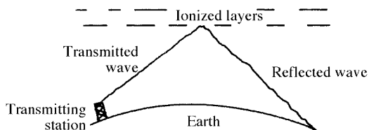
atmospheric reflection
