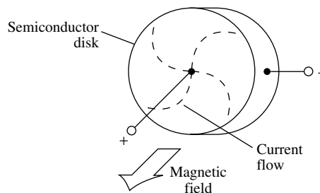
Corbino effect
