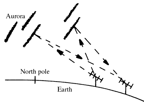
auroral propagation
