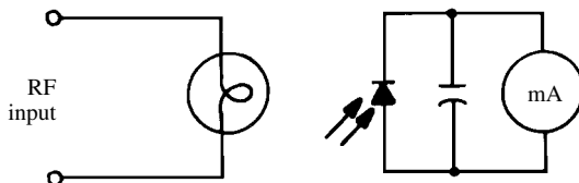
photoelectric wattmeter
