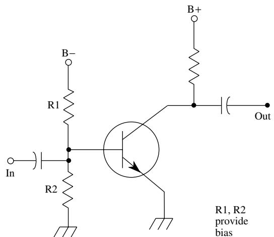
back bias, 3
