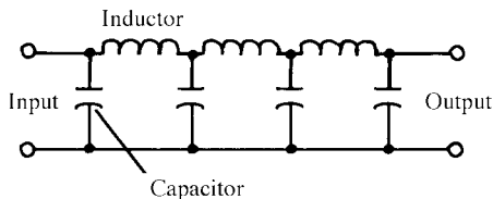
artificial transmission line
