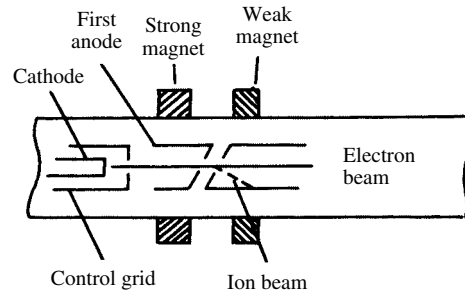
slashed-field-gun CRT
