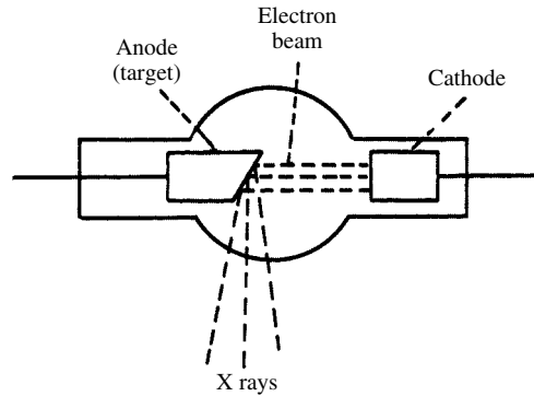
X-ray tube
