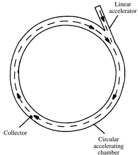
synchrotron
