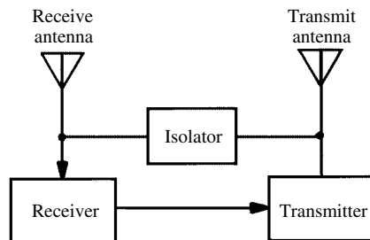
repeater
