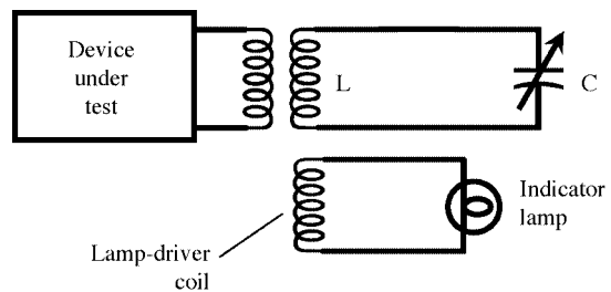
absorption wavemeter
