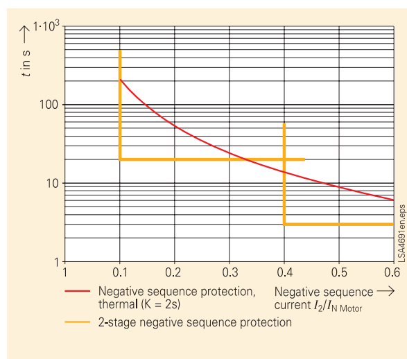
Fig. 9 Negative-sequence protection characteristics
