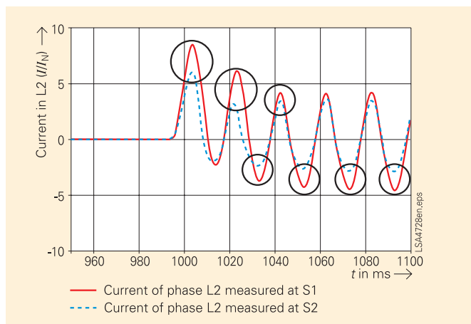
Fig. 5 Depiction of the reason for the differential current transformer saturation in phase L2 of side 2 (evaluated with Mathcad)
