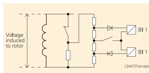
Fig. 3 Circuit for evaluating the rotor voltage
