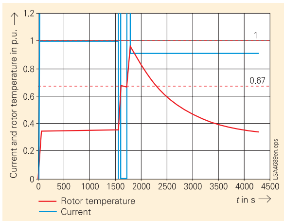
Fig. 7 Behavior under different loads according to the thermal rotor model ( t_{\text{start}} = 52 \text{ s} ; I_{\text{start}} = 4.17 // I_{N,M} ; n_c = 3 and n_w = 2 )
